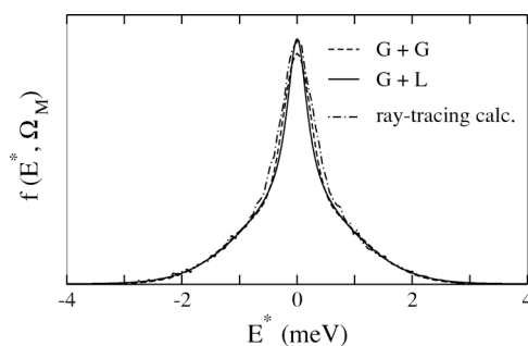
FIG. 3. Derived resolution function f(E^*, \Omega_M) of the PGM monochromator, E^*=E'-E'' is the energy with respect to the monochromator energy E' , G+G represents one monochromator-resolution model given by the sum of two Gaussians, while G+L stands for the other model given by the sum of a Gaussian and a Lorentzian function. The dash-dotted curve represents the results of ray-tracing simulations (see text).
