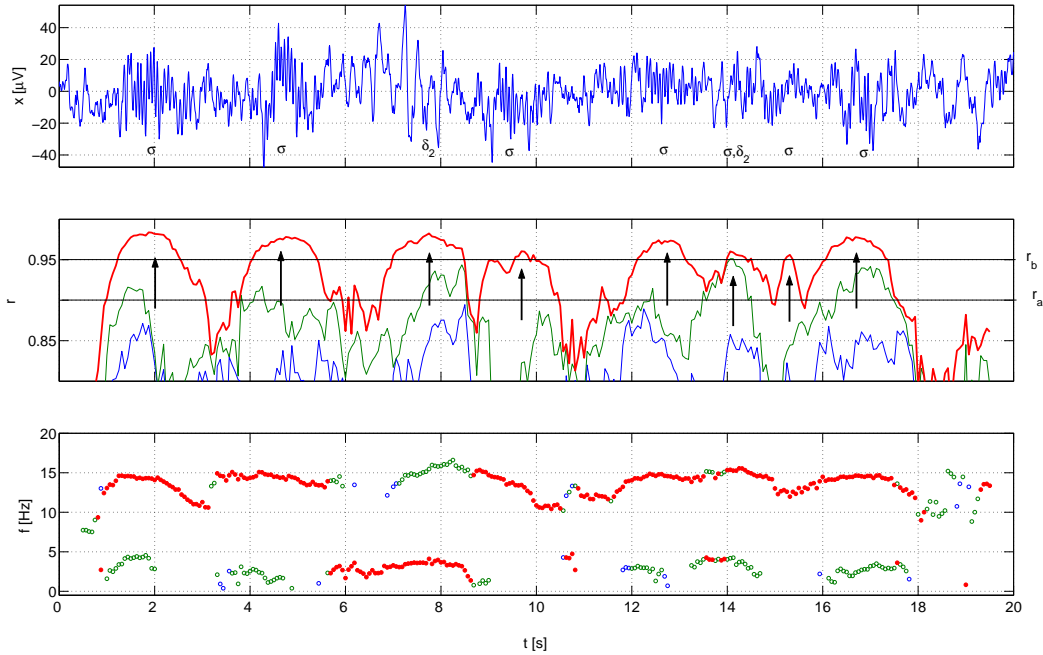
Fig. 1. EEG data (upper panel) with oscillatory events marked by arrows, \sigma -spindles and \delta_2 - fast delta waves. The time course of r_k and the corresponding frequencies f_k are shown in the lower panels. The pole with lowest damping is indicated by the bold red line and filled circles, the poles with the second and third lowest damping by the green and blue lines and circles, respectively.
